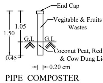
PIPE COMPOSTER
