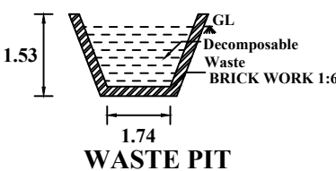
WASTE PIT
