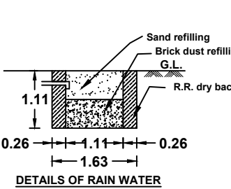
DETAILS OF RAIN WATER HARVESTING
