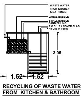
RECYCLING OF WASTE WATER FROM KITCHEN & BATHROOM
