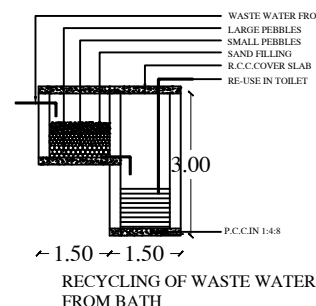
RECYCLING OF WASTE WATER FROM BATH
