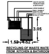
RECYCLING OF WASTE WATER FROM KITCHEN & BATHROOM
