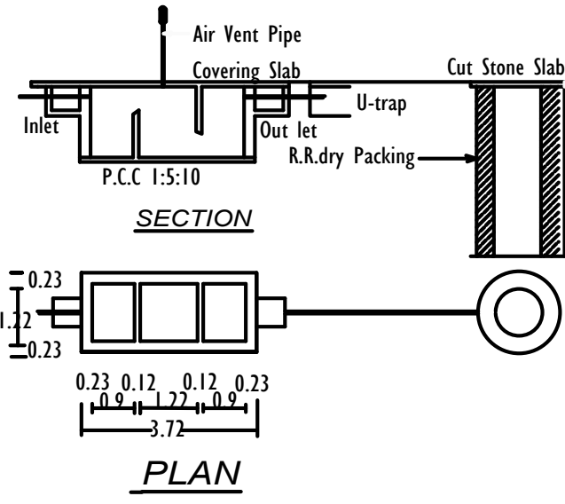
SEPTIC TANK DETAILS SCALE 1cm : 1m
