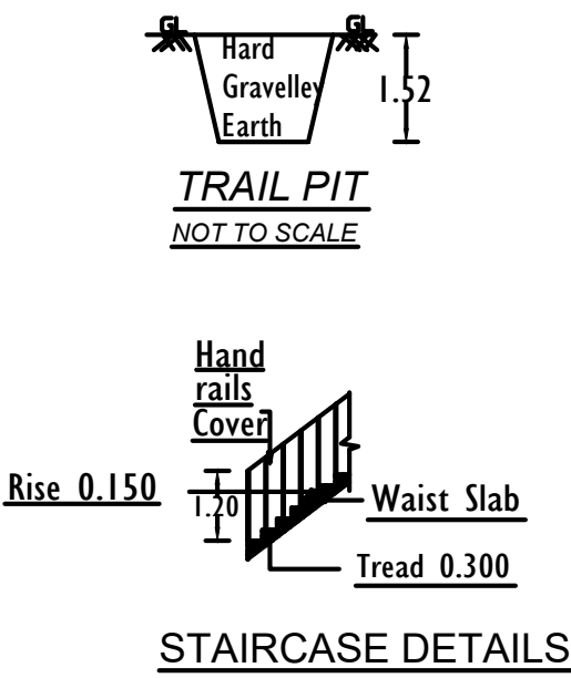
STAIRCASE DETAILS
