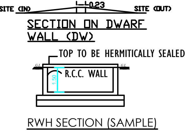
RWH SECTION (SAMPLE)
