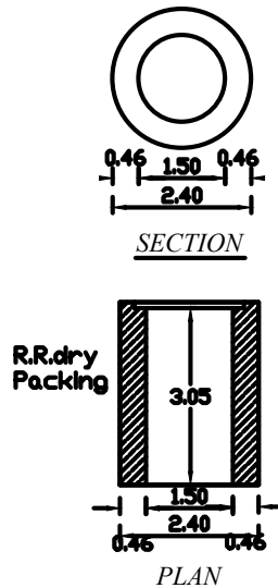
RAIN WATER HARVESTING ARRANGEMENT NOT TO SCALE
