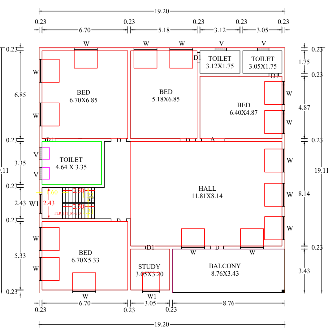
PLAN OF SECOND FLOOR
