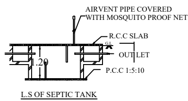
L.S. OF SEPTIC TANK
