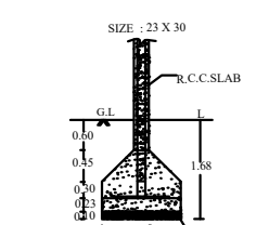
DETAILS OF R.C.C. COLUMN
