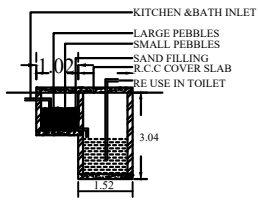
DETAILS OF RECYCLING OF WASTE
