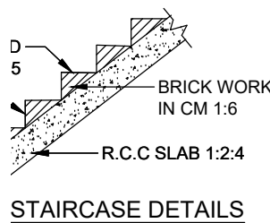
STAIRCASE DETAILS
