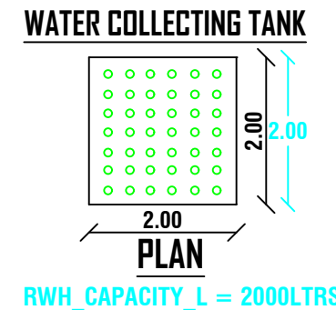
WATER COLLECTING TANK
