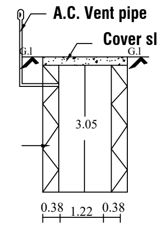
Soakpit section
