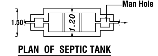
PLAN OF SEPTIC TANK
