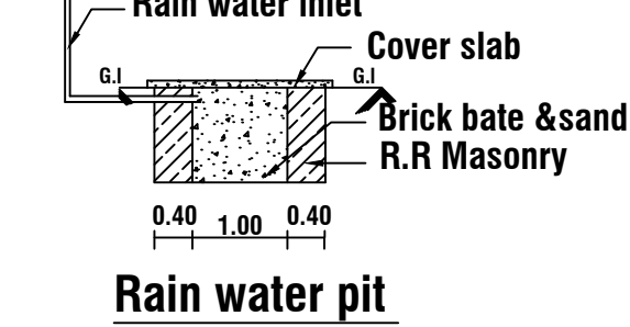
Rain water pit
