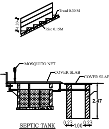
SEPTIC TANK
