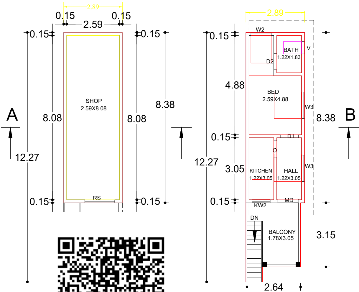
FIRST FLOOR PLAN (RESIDENTIAL BUILDING)
