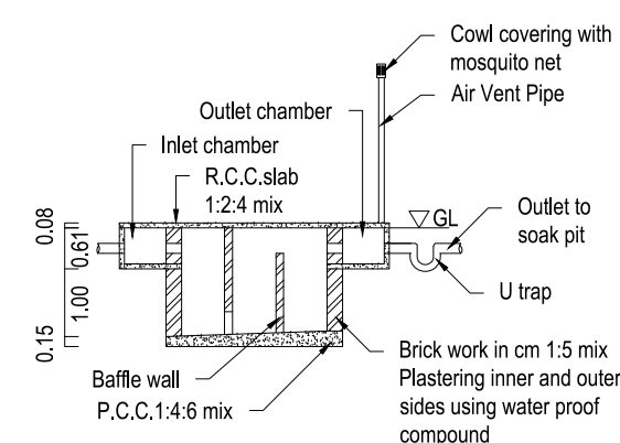
SECTION UV
