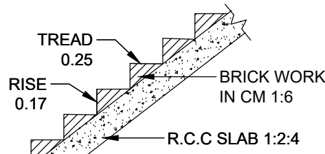
STAIRCASE DETAILS
