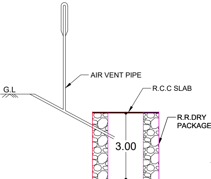
SECTION OF SOAKPIT
