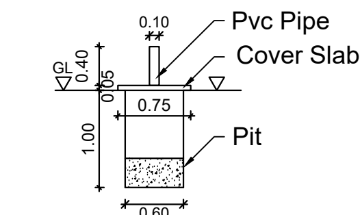
SOLID WASTE COMPOST PIT
