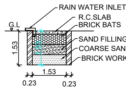
RAIN WATER HARVESTING PIT RW_H_CAPACITY_L=5000LTRS
