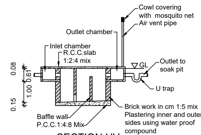
SECTION UV
