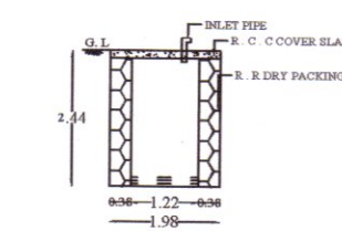
RAIN WATER STORAGE TANK SECTION
