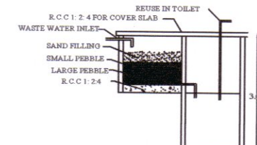
RECYCLING OF WASTE WATER
