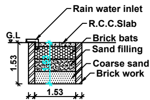
RAIN WATER HARVESTING PIT RWH_CAPACITY_L=5000LTRS
