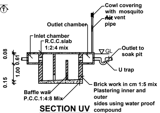
SECTION UV
