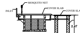
SEPTIC TANK
