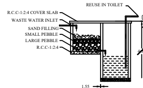
RECYCLING OF WASTE WATER KITCHEN & BATH ROOM
