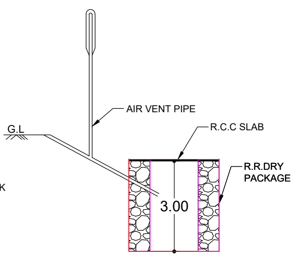
SECTION OF SOAKPIT
