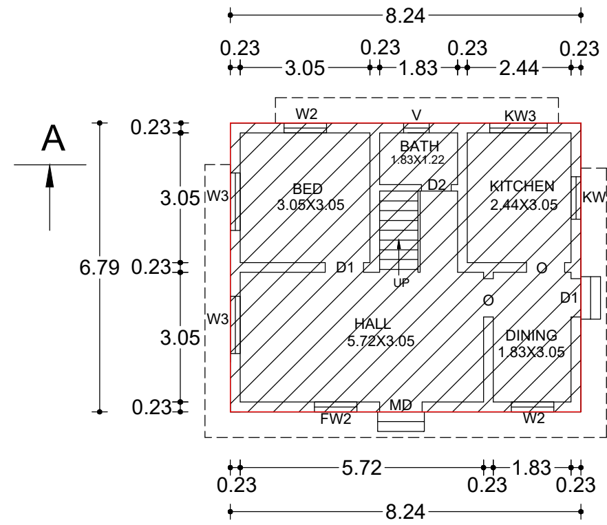
EXG.GROUND FLOOR PLAN
