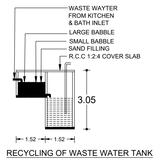
RECYCLING OF WASTE WATER TANK
