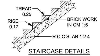
STAIRCASE DETAILS
