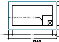
SEPTIC TANK DETAILS
