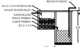
RECYCLING OF WASTE WATER KITCHEN & BATH ROOM
