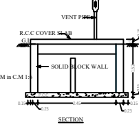
SOAK PIT (NOT TO SCALE)
