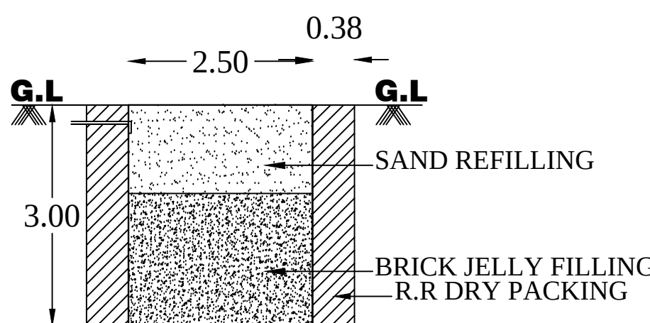
RAINWATER HARVESTING
