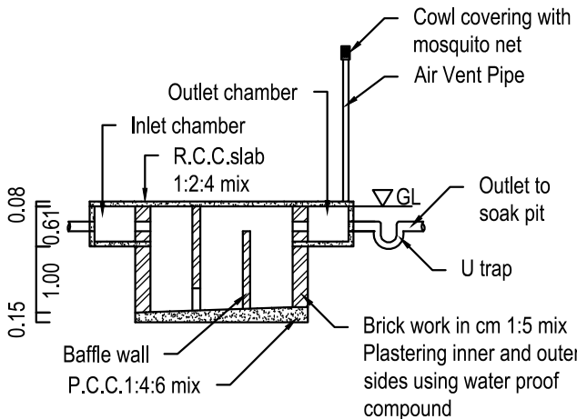
SECTION UV
