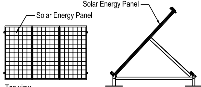
SOLAR POWER SYSTEM
