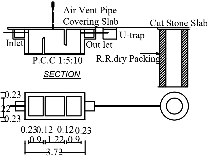
PLAN SEPTIC TANK DETAILS SCALE 1cm : 1m
