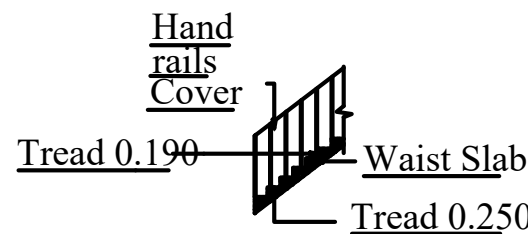
STAIRCASE DETAILS
