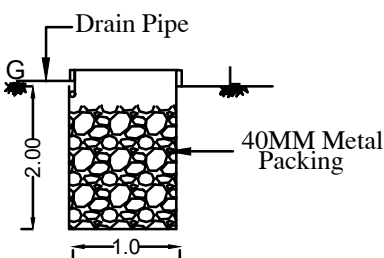
RAIN WATER SYSTEM
