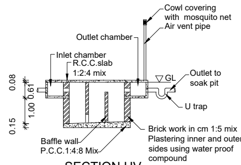
SECTION UV
