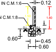
COMPOUND WALL SECTION
