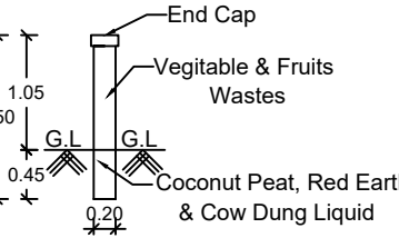
PIPE COMPOSTER
