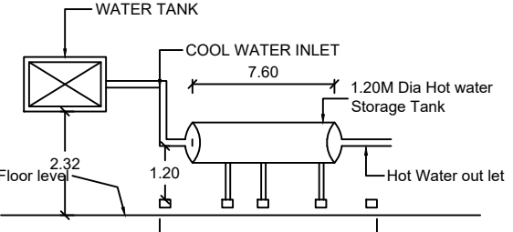
SOLAR WATER HEATING SYSTEM (S.W.H.S.DETAILS)
