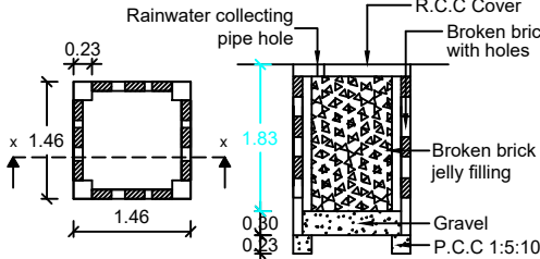
PLAN RAIN WATER HARVEST WELL
