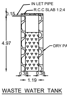
WASTE WATER TANK
