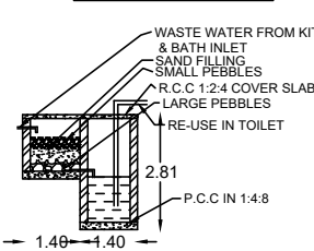
RECYCLING OF WASTE WATER KITCHEN & BATHROOM
