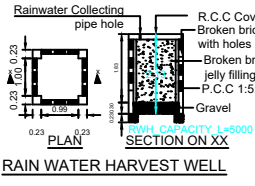
RAIN WATER HARVEST WELL
