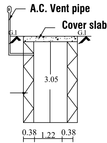
Soakpit section
