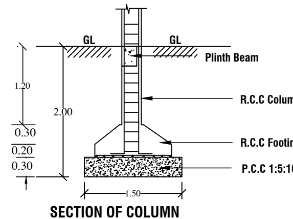
SECTION OF COLUMN
