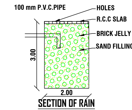
SECTION OF RAIN
