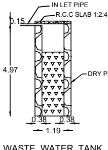
WASTE WATER TANK
