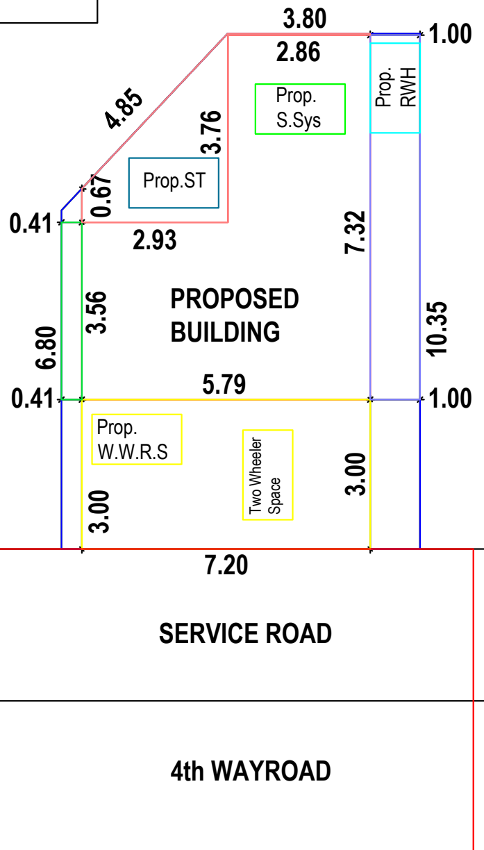
SITE PLAN
