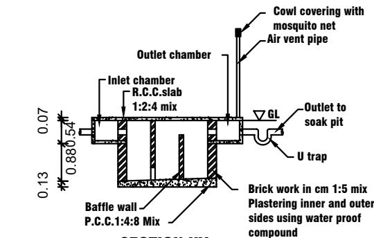
SECTION UV
