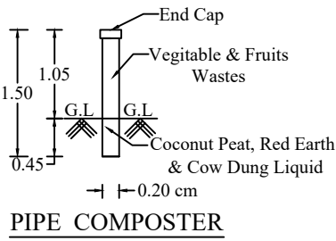
PIPE COMPOSTER
