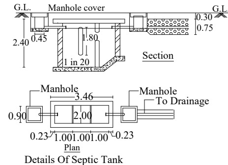
Details Of Septic Tank
