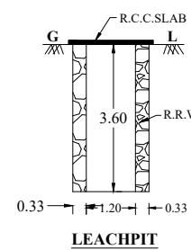
LEACHPITT
