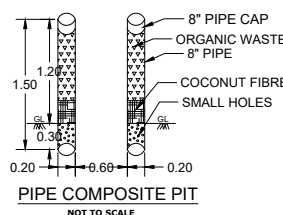
PIPE COMPOSITE PIT NOT TO SCALE
