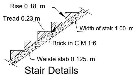
Stair Details
