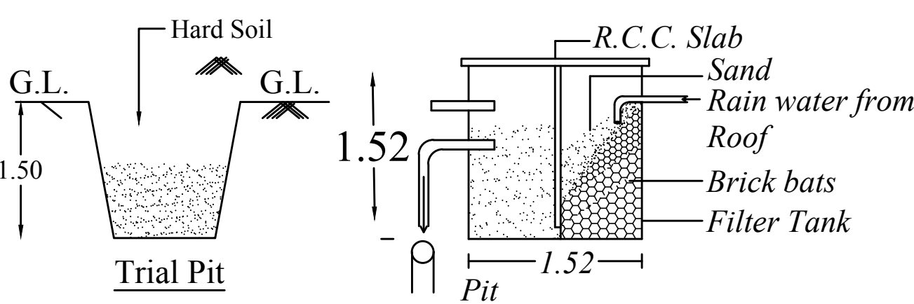
Rain Water Storage
