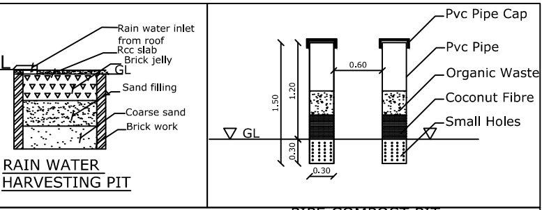
PIPE COMPOST PIT
