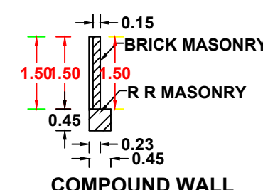
COMPOUND WALL
