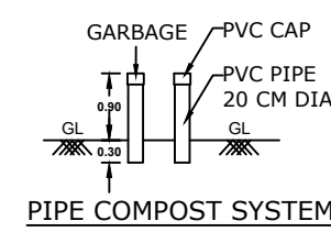
PIPE COMPOST SYSTEM
