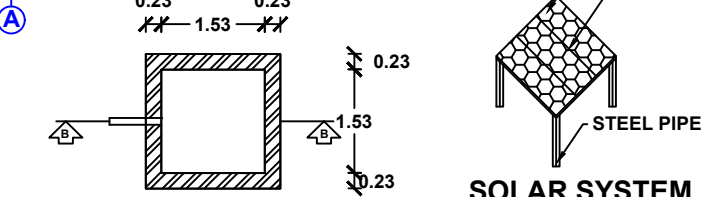
PLAN OF RAIN WATER HARVESTING TANK
