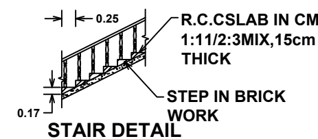
STAIR DETAIL
