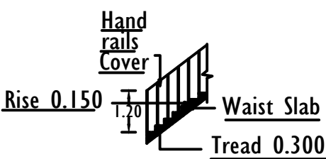
STAIRCASE DETAILS
