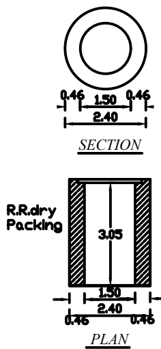
RAIN WATER HARVESTING ARRANGEMENT
