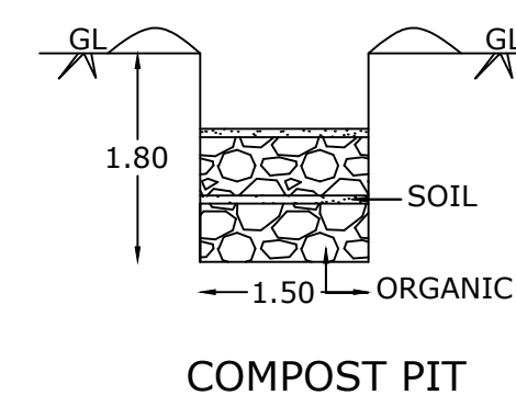
COMPOST PIT
