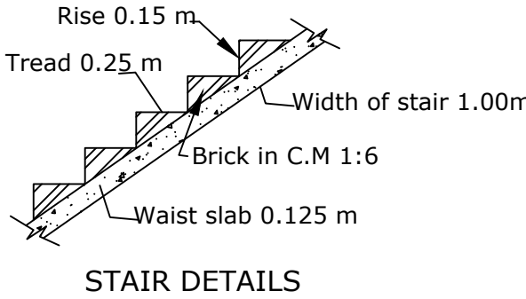
STAIR DETAILS
