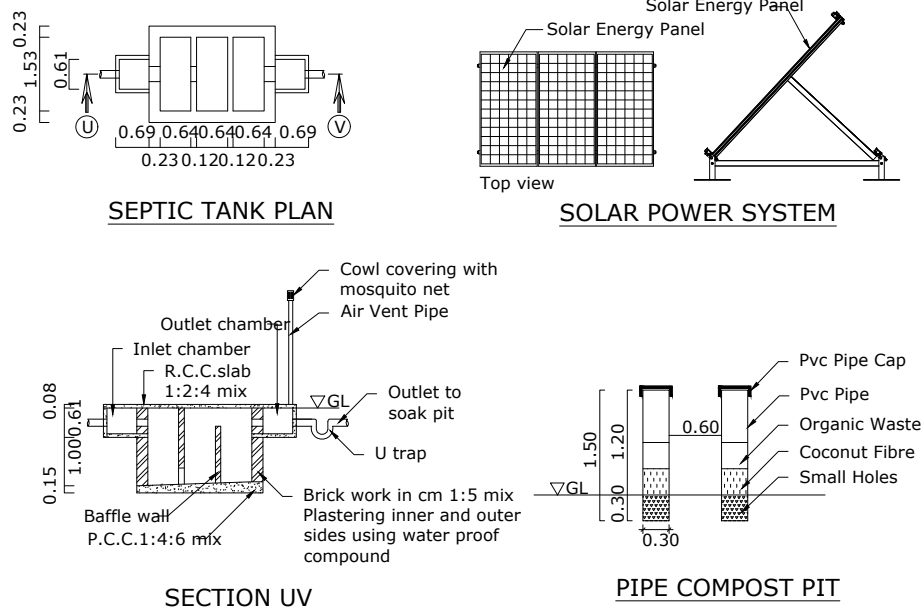
SECTION UV
