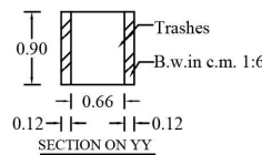
SECTION ON 'YY'
