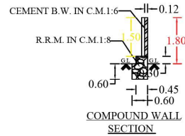
COMPOUND WALL SECTION
