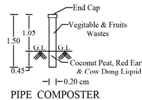
PIPE COMPOSTER
