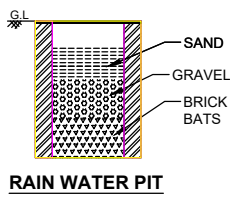
RAIN WATER PIT
