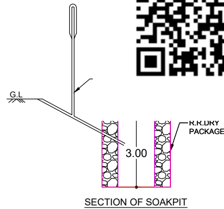
SECTION OF SOAKPIT
