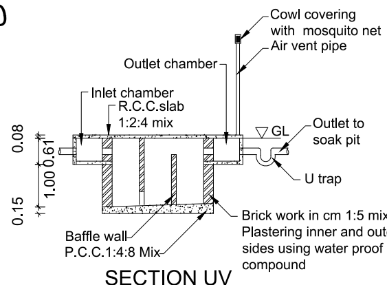
SECTION UV
