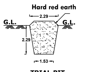
TRIAL PIT
