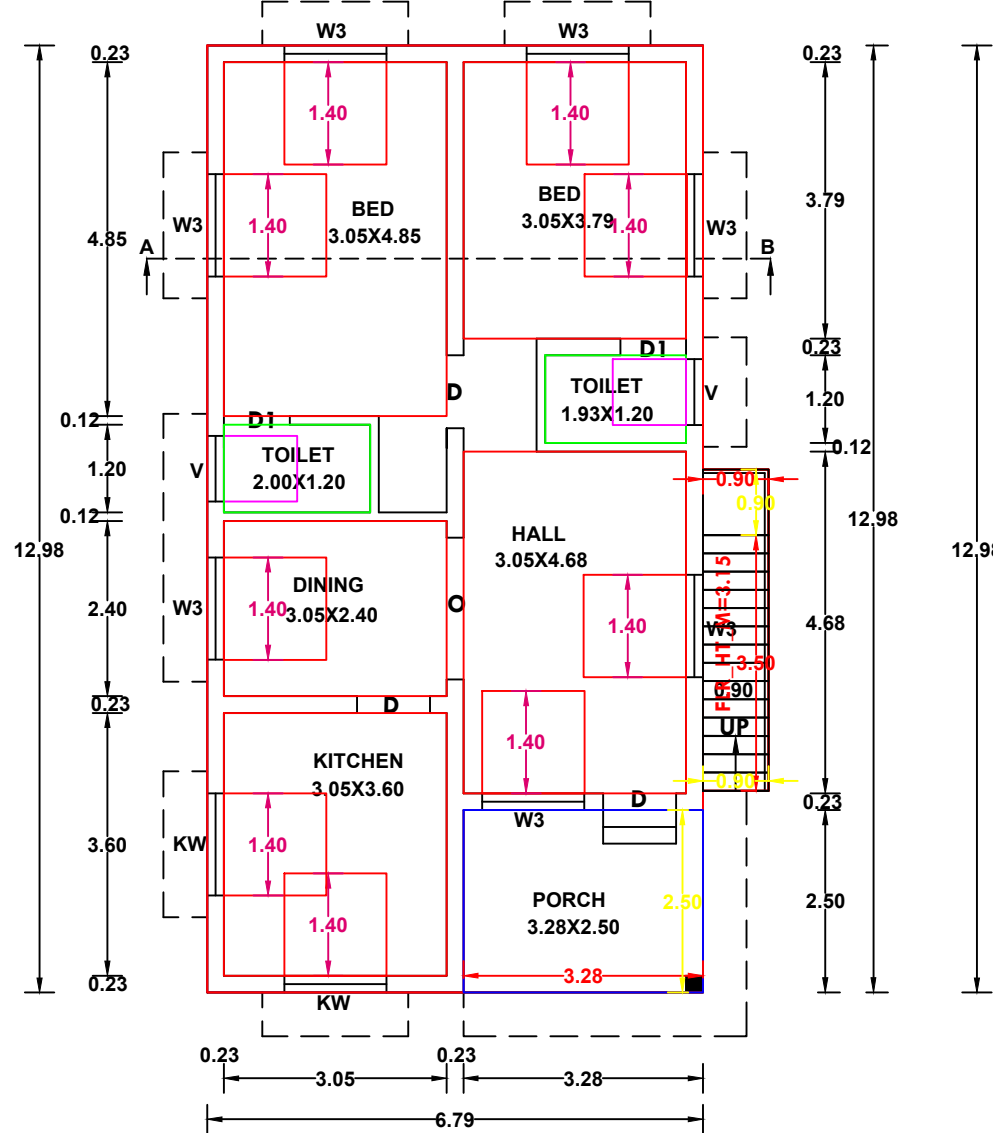
GROUND FLOOR PLAN(HOUSE-1)
