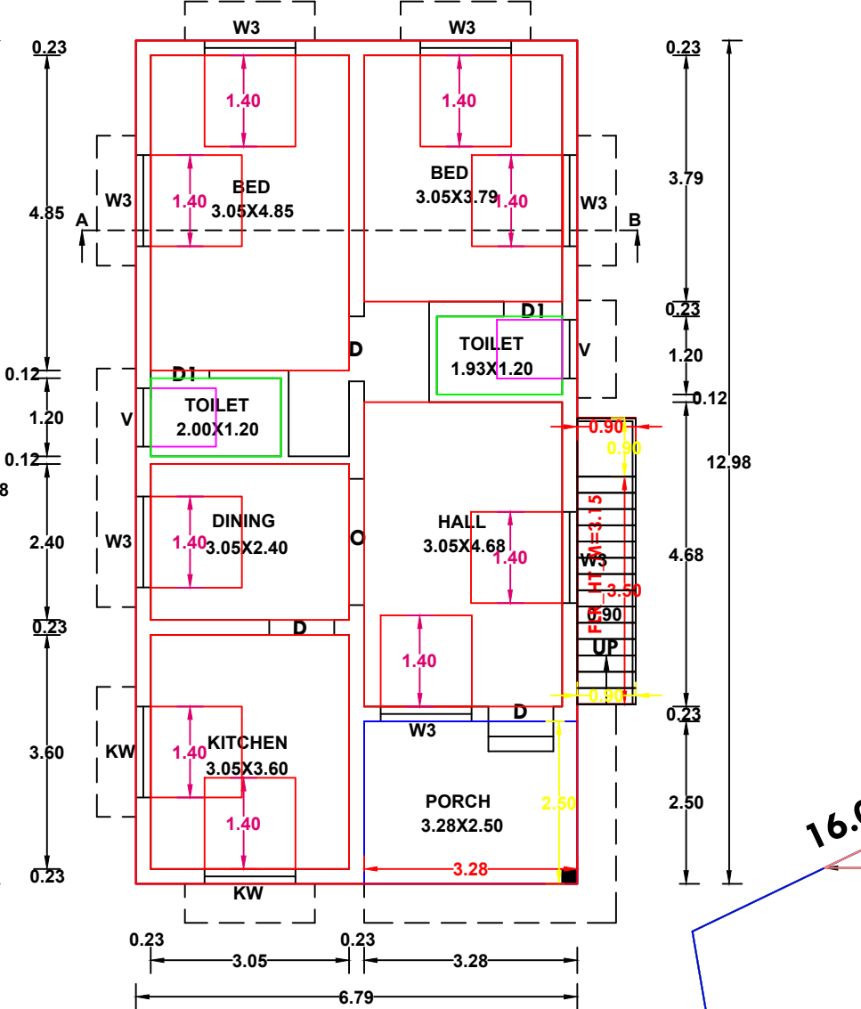
GROUND FLOOR PLAN(HOUSE-2)
