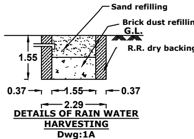
DETAILS OF RAIN WATER HARVESTING Dwg: 1A
