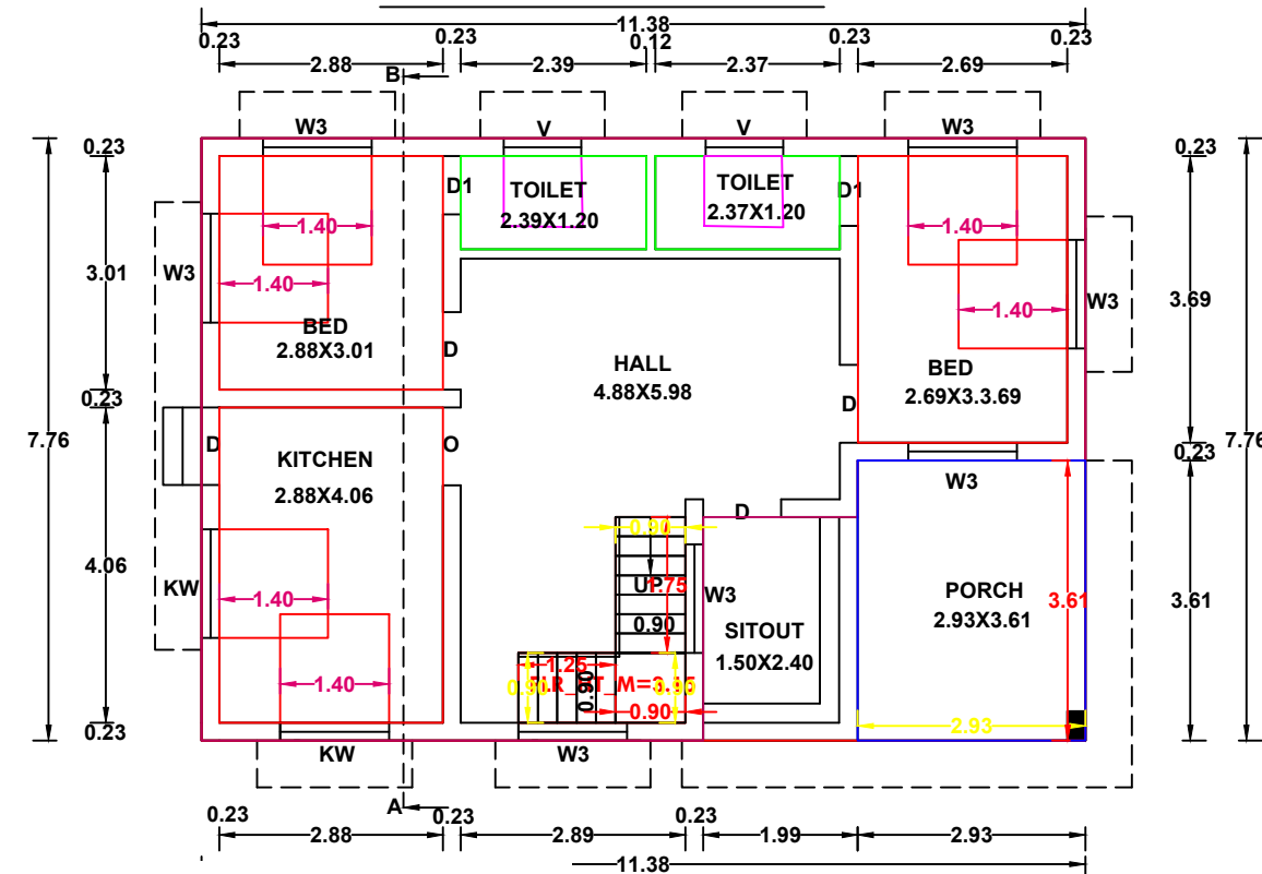
ND FLOOR PLAN
