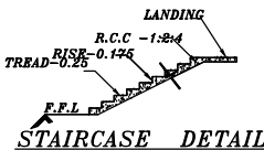
STAIRCASE DETAIL
