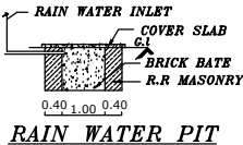
RAIN WATER PIT
