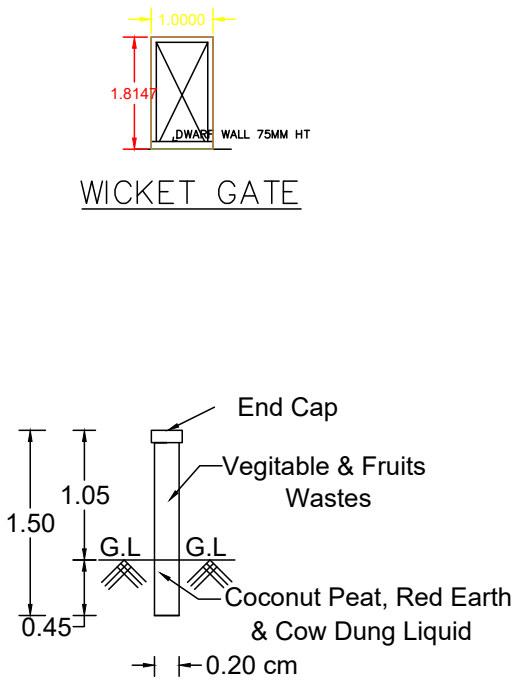
PIPE COMPOSTER
