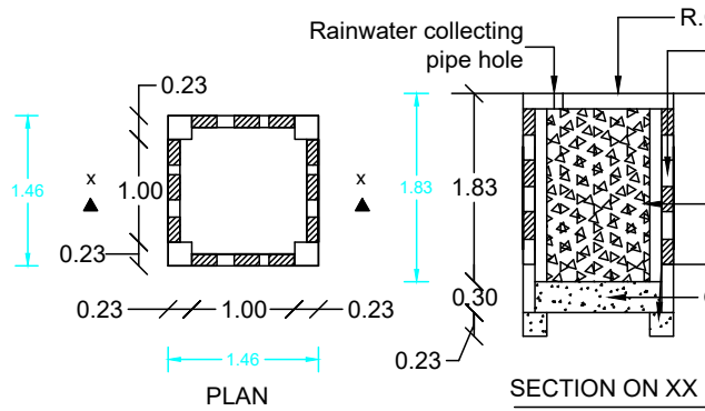
RAIN WATER HARVEST WELL
