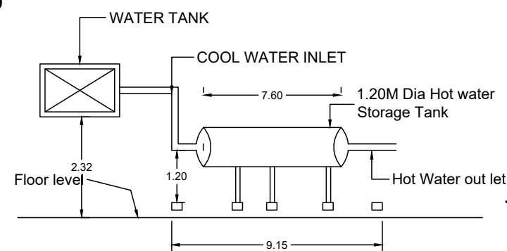
SOLAR WATER HEATING SYSTEM (S.W.H.S.DETAILS)
