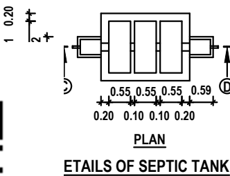
DETAILS OF SEPTIC TANK
