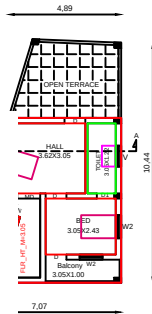
2ND FLOOR PLAN
