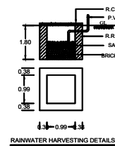
RAINWATER HARVESTING DETAILS
