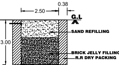
RAINWATER HARVESTING
