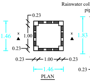
RAIN WATER HARVEST WELL
