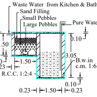
WASTE WATER RECYCLING SYSTEM
